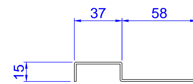
Standard 15mm STEEL
