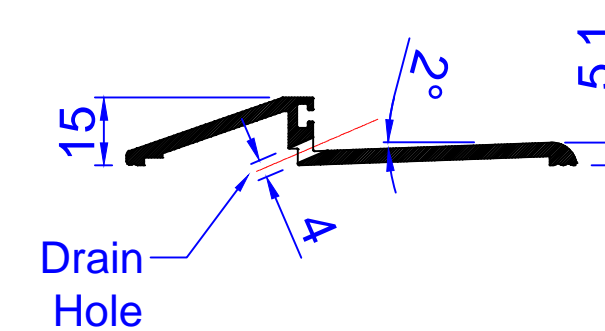
15mm ALUMINIUM (INWARD OPENING)
