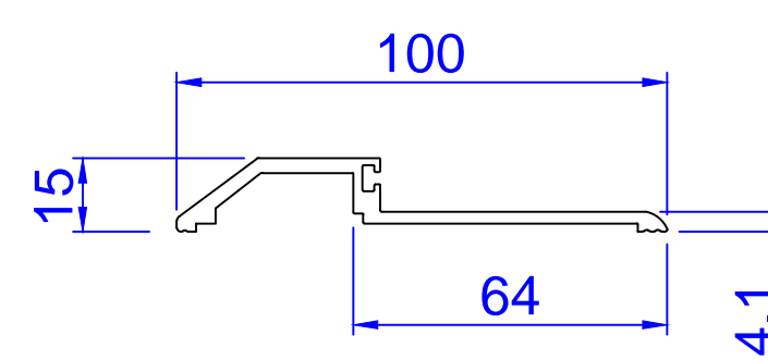
Zero 564 15mm ALUMINIUM
